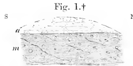
Fig. 1.† a. Gravel horizontally stratified. 10 feet? m. Light grey loam with angular débris and blocks in inclined rough bedding. 20 feet?
